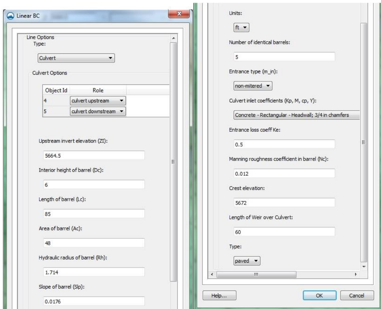
Figure 5 Culvert Parameters
