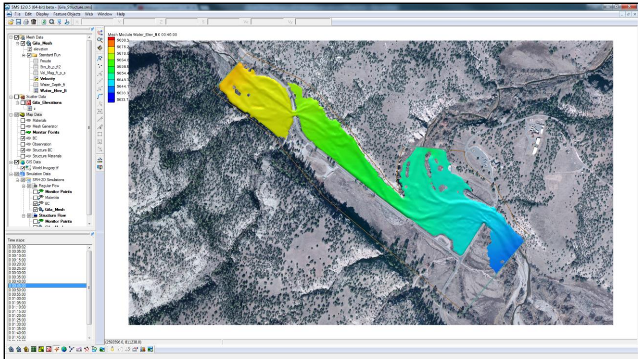
Figure 1 Gila_Structure.sms project
