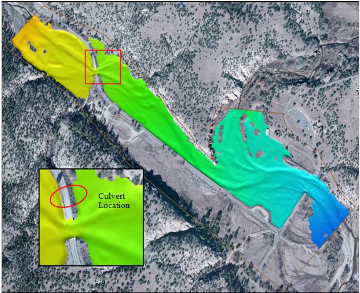
Figure 2 Culvert location
